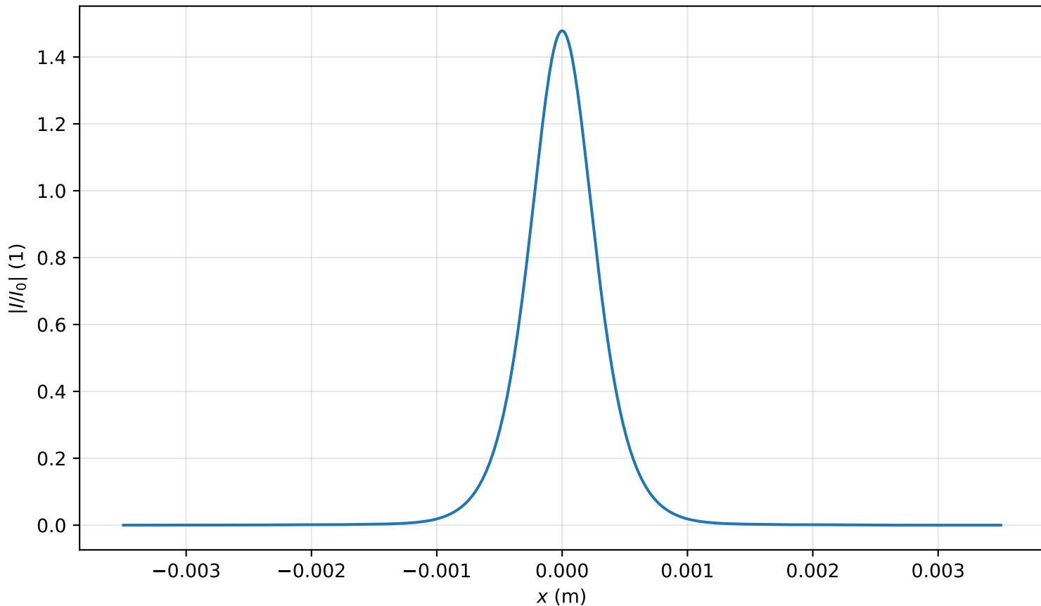
Intensity profile I(x, y = 0, z = 3.582m)/I_0 , P_{in}=0.9P_{cr} , artificial time
